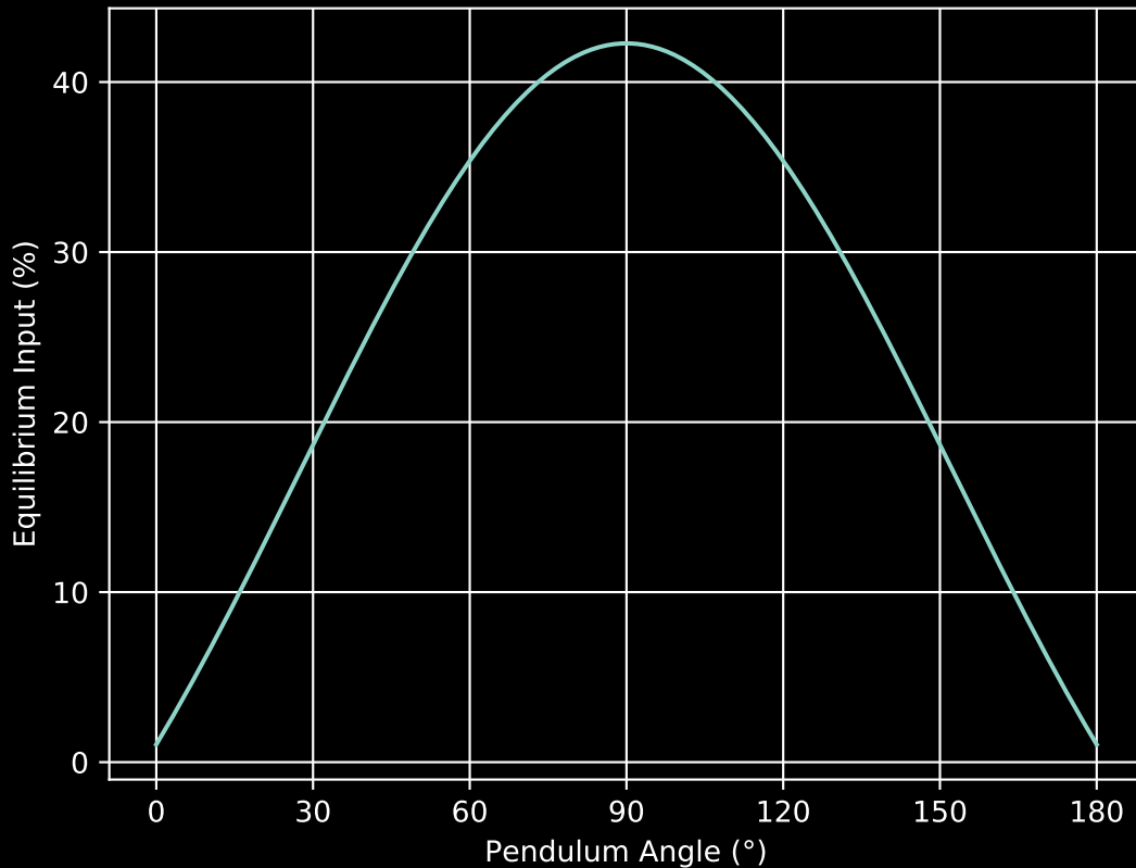
Required input for force equilibrium as function of pendulum angle
